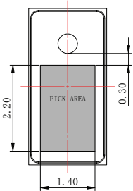
Recommended Vacuum Nozzle Pickup Top View
