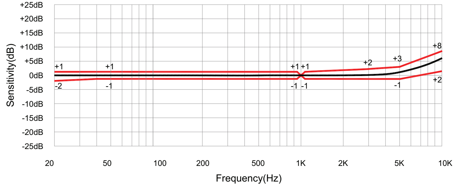
Frequency Response (0dB=1V/Pa)
