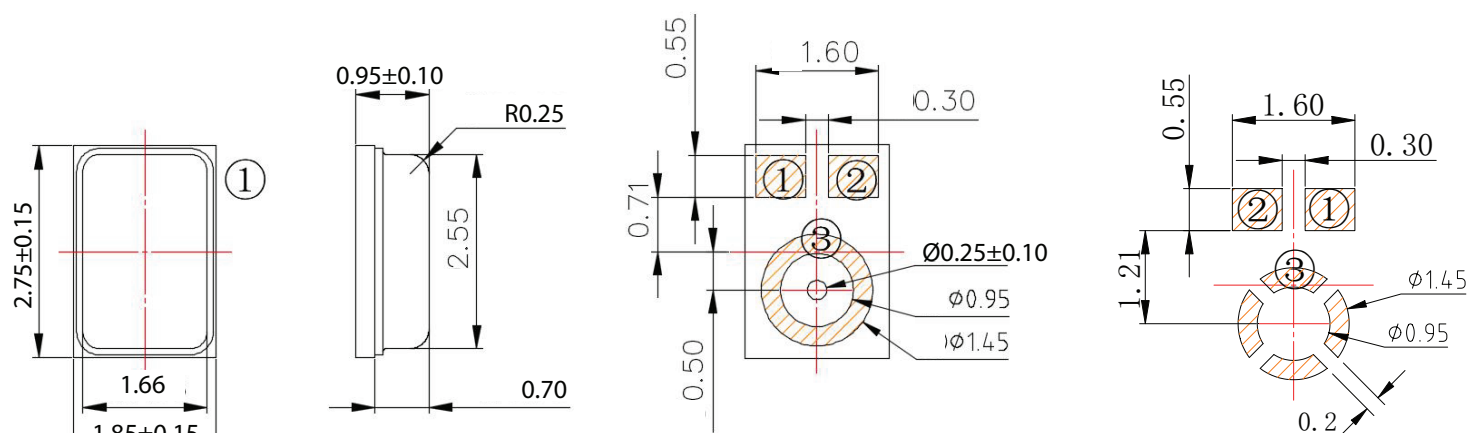
Recommended Stencil Pattern Top View
