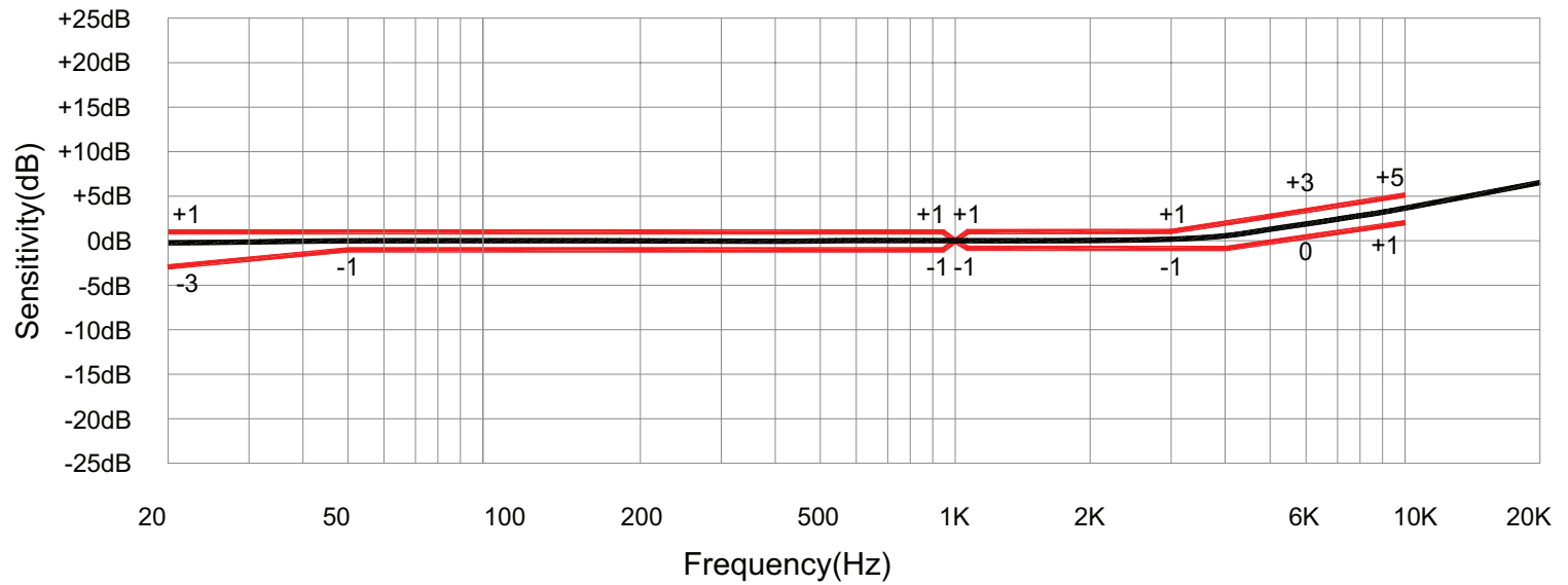
Frequency Response (0dB=1V/Pa)
