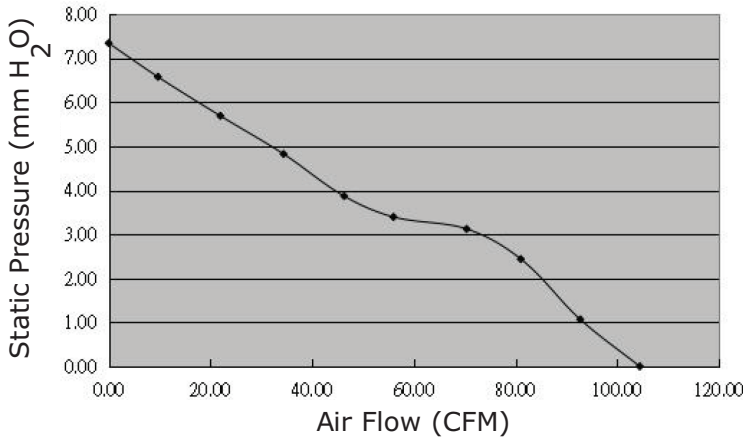
CFM-A225BG-423-386
