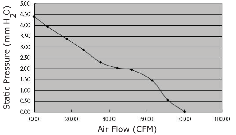
CFM-A225BG-415-267
