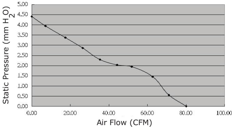
CFM-A225BG-423-386
