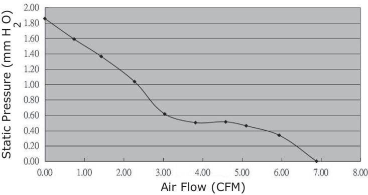
CFM-5015CG-060-302
