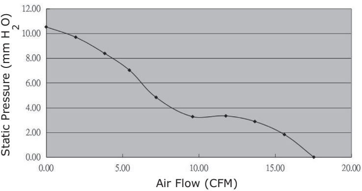
CFM-5015CG-075-366
