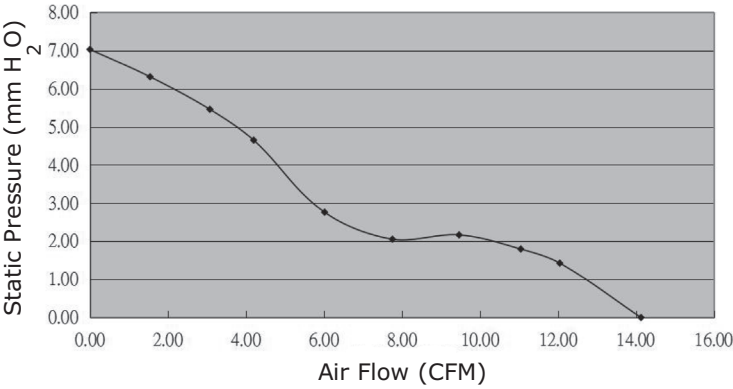
CFM-5015CG-060-302
