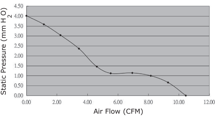
CFM-5015CG-075-366
