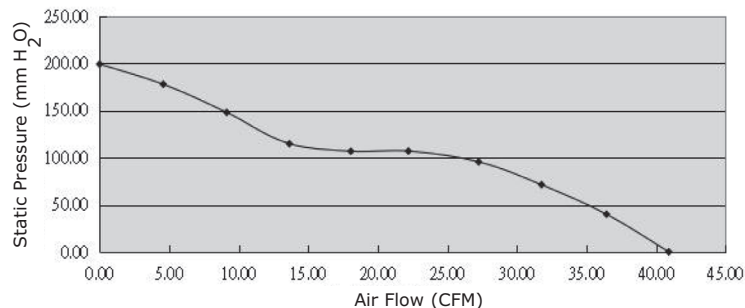
CFM-4028BH-1350-689
