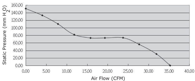
CFM-4028BH-1300-653
