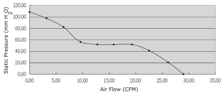
CFM-4028BH-1250-622
