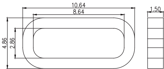
O-ring (P/N: OR-140)
