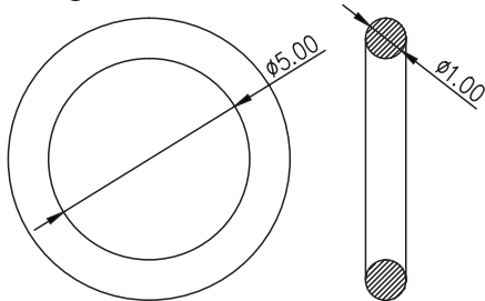
O-ring (P/N: OR-150)
