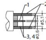
MATING PLUG Jack Insertion Depth: 9.1 mm
