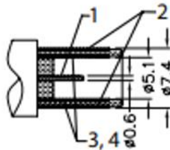
MATING PLUG Jack Insertion Depth: 9 mm
