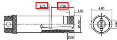
MATING PLUG Jack Insertion Depth: 9.5 mm
