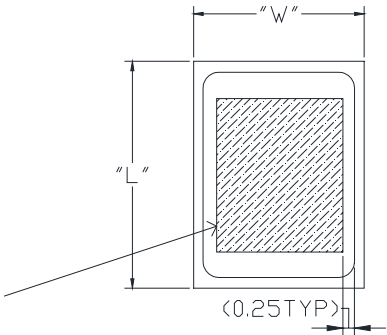
Recommended Vacuum Nozzle Pickup Top View
